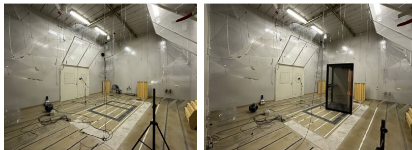
Measurement of T_0 and T_1 according to ISO354.
