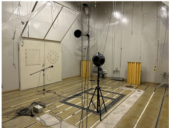
Picture 3 and 4: Loudspeaker and Microphones for L_{W0} measurements All in all 2 loudspeaker positions and 8 microphone positions for each one of these.
