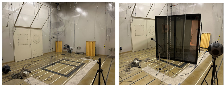
Measurement of T_0 and T_1 according to ISO354.
